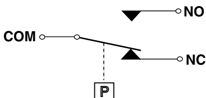
Diagram Shows Pressure Being Applied To Switch
